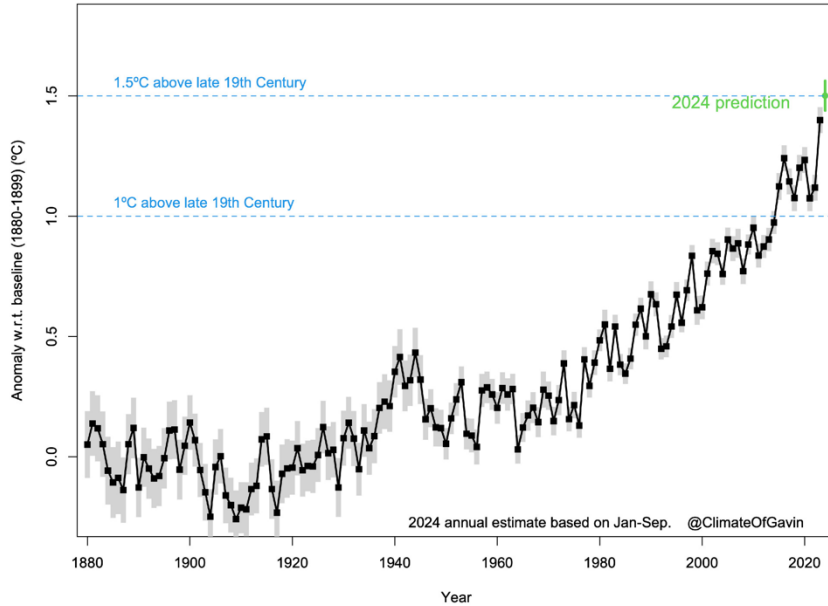
GISTEMP v4 LOTI (incl. 2024 prediction)
